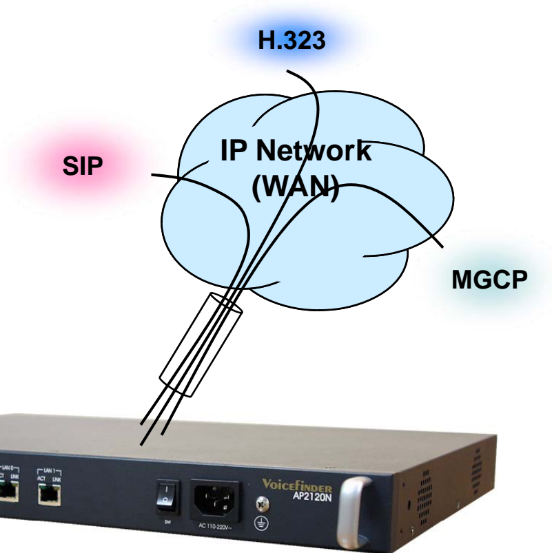
Concurrent Triple VoIP Stack
