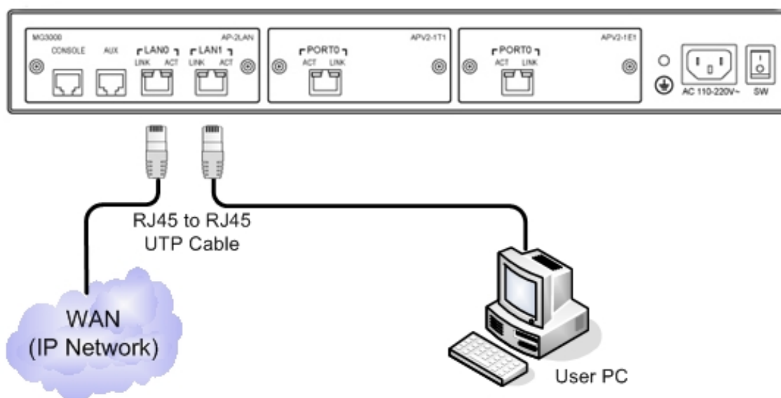
[ Figure 3-2 Connection between AP-MG3000N LAN0/LAN1 and WAN equipment/PC ]
