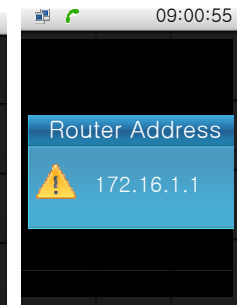
4) Router Address
