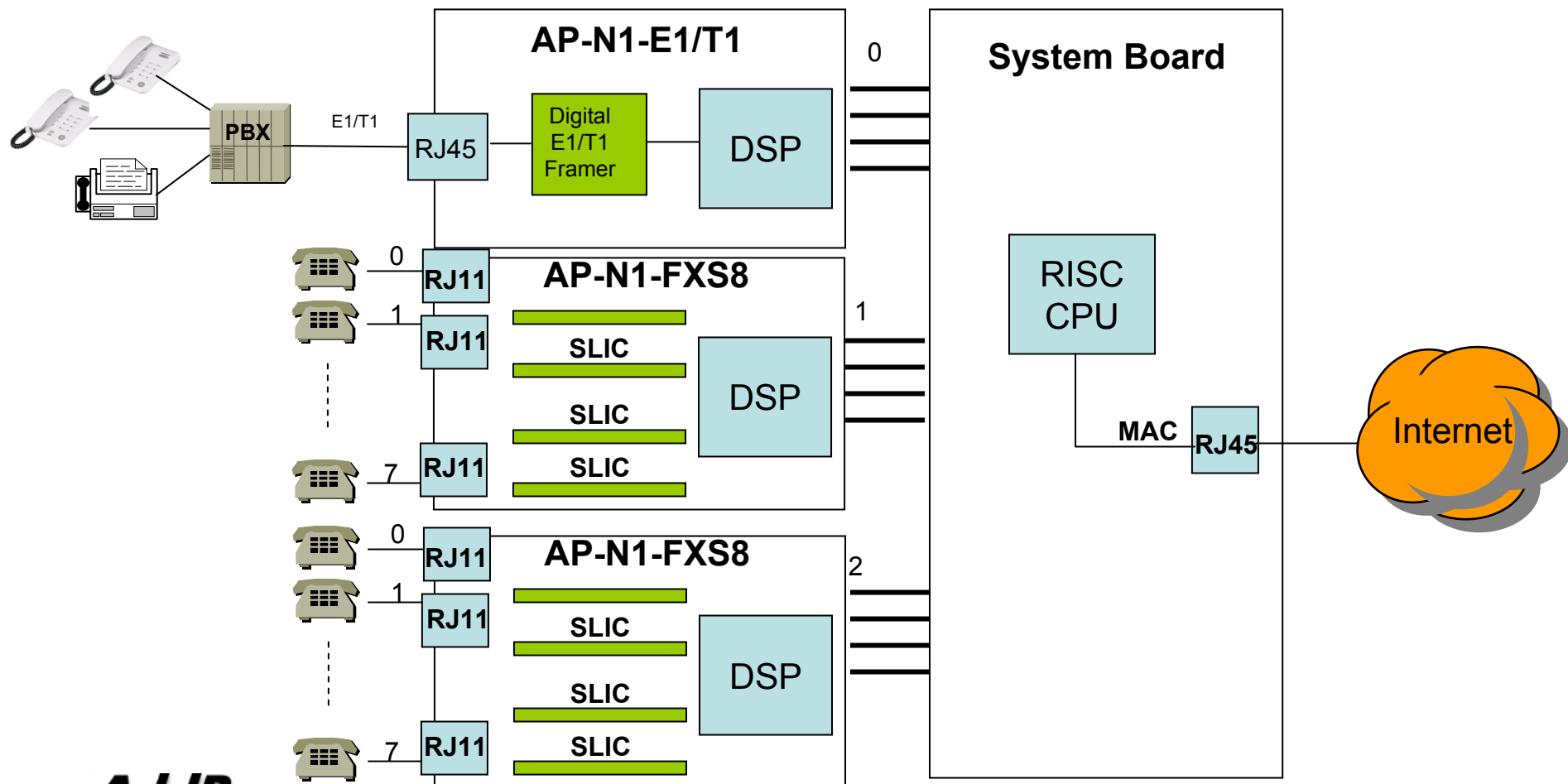
16-Port FXS+ 1-Port Digital E1/T1 Service Diagram
