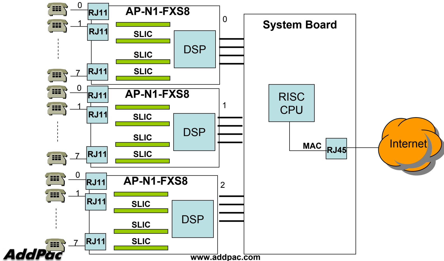
24-Port(8x3Module) FXS Gateway Service Diagram
