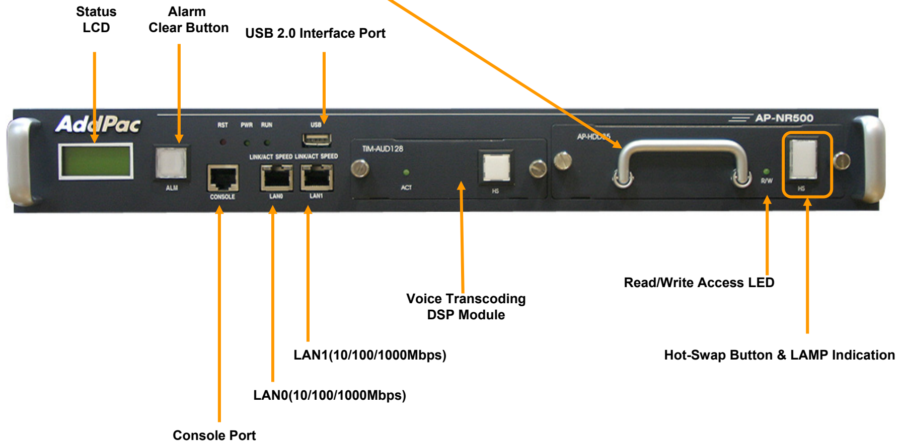
AP-NR500 Front Side
