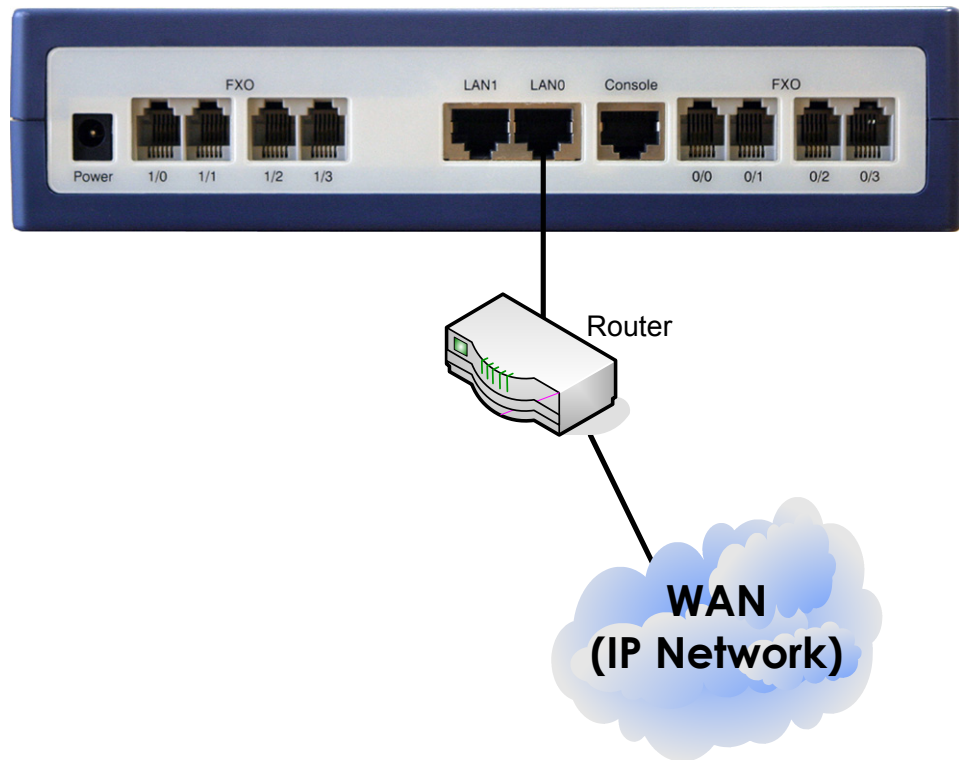
Figure 3-2: Network connection diagram between AP1100F gateway and WAN network
