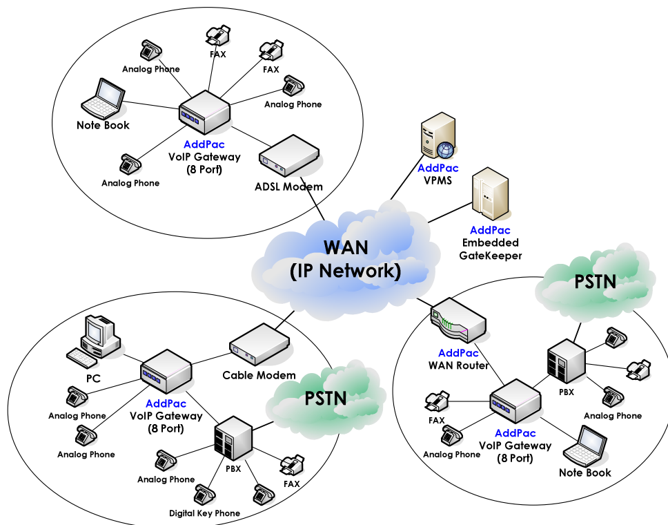
Figure 1-1: The network diagram using VoiceFinder AP1100F Gateway
