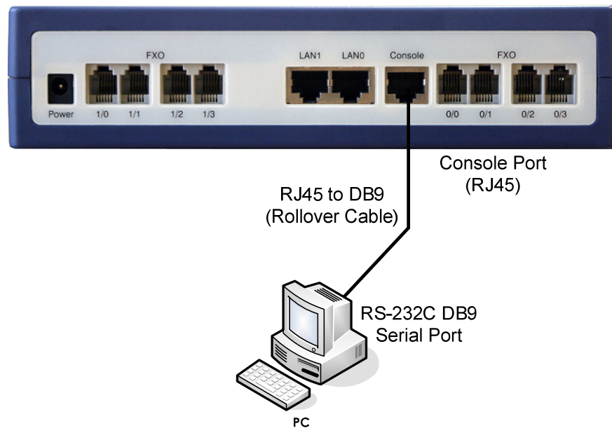
Figure 3-1: RS-232C Console port interface diagram between AP1100F VoIP gateway and PC or notebook computer
