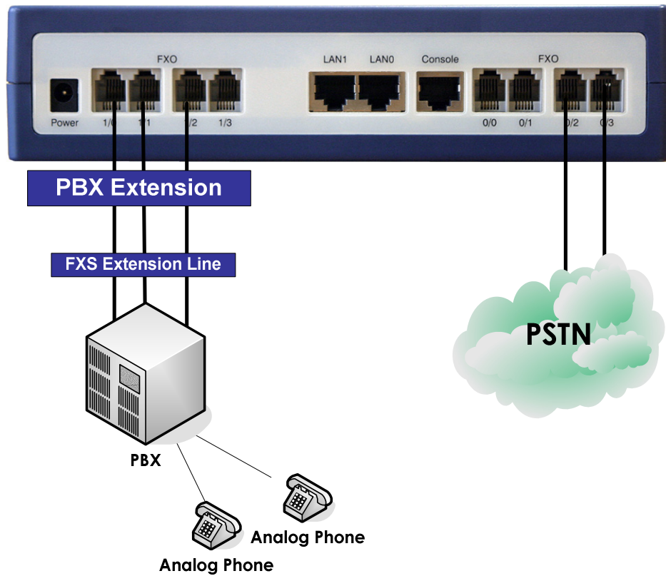
Figure 3-4: FXO analog voice port interface diagram between AP1100F VoIP gateway and PBX or PSTN
